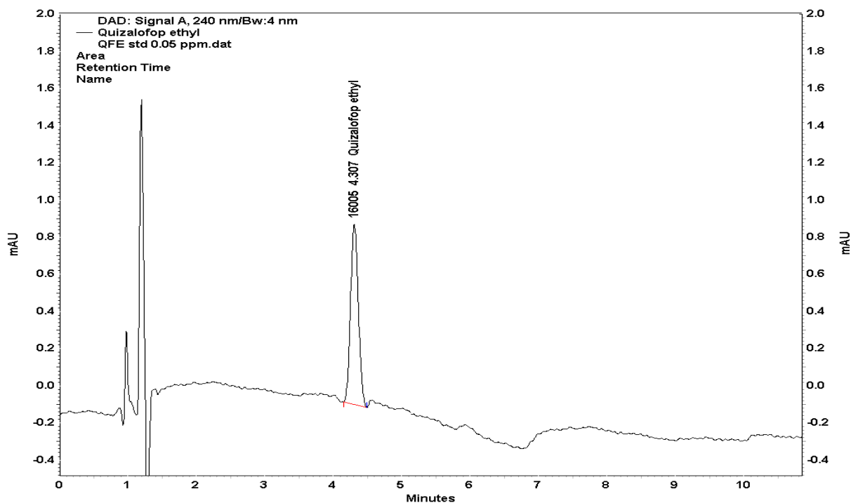
Figure 2- HPLC chromatograms of standard quizalofop ethyl at 0.05 µg mL -1
